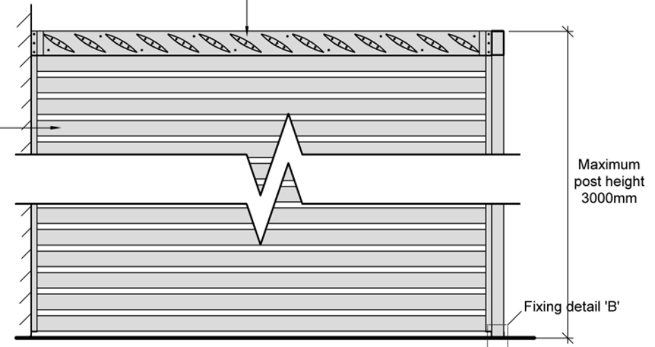
SECTION DETAIL
