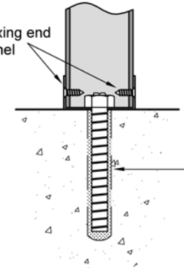
FIXING DETAIL 'B'
