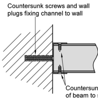
FIXING DETAIL 'A'
